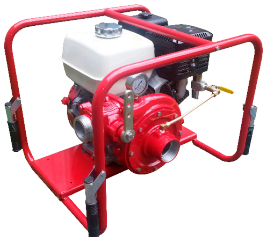
PFP-11hp-HND-M
