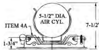
TOP VIEW RECESSED PLATFORM MODEL MQSD/U
